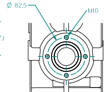
OUTPUT FLANGE
